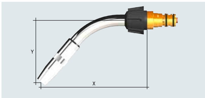
removable and rotateable torch necks.
